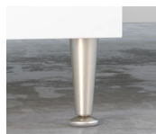
S: Round
